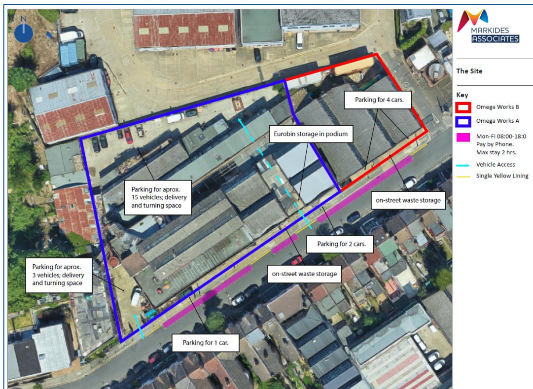
Figure 3.2 Existing Site
