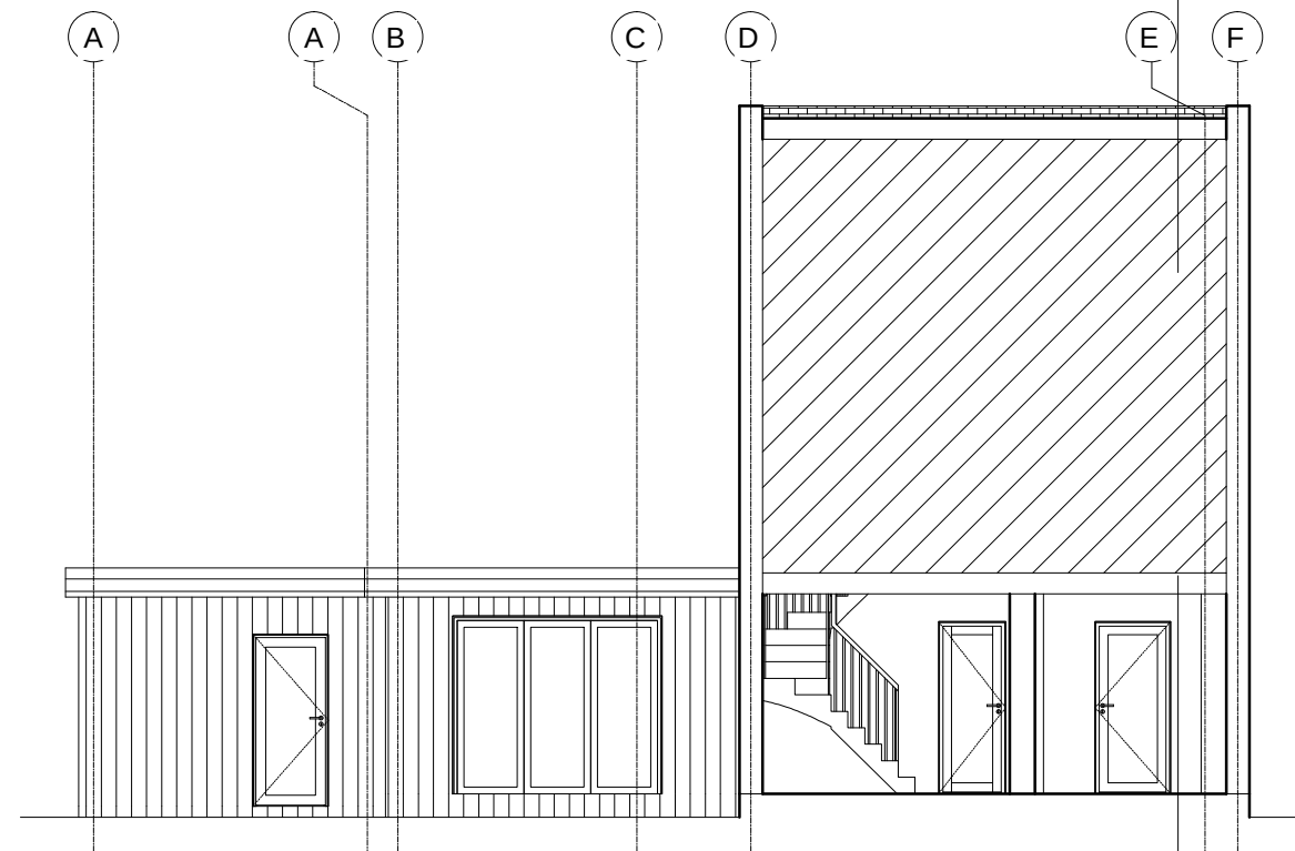
PROPOSED SECTION B
