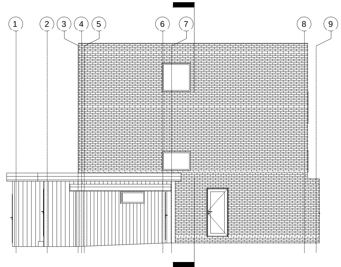
EXISTING LEFT SIDE ELEVATION
