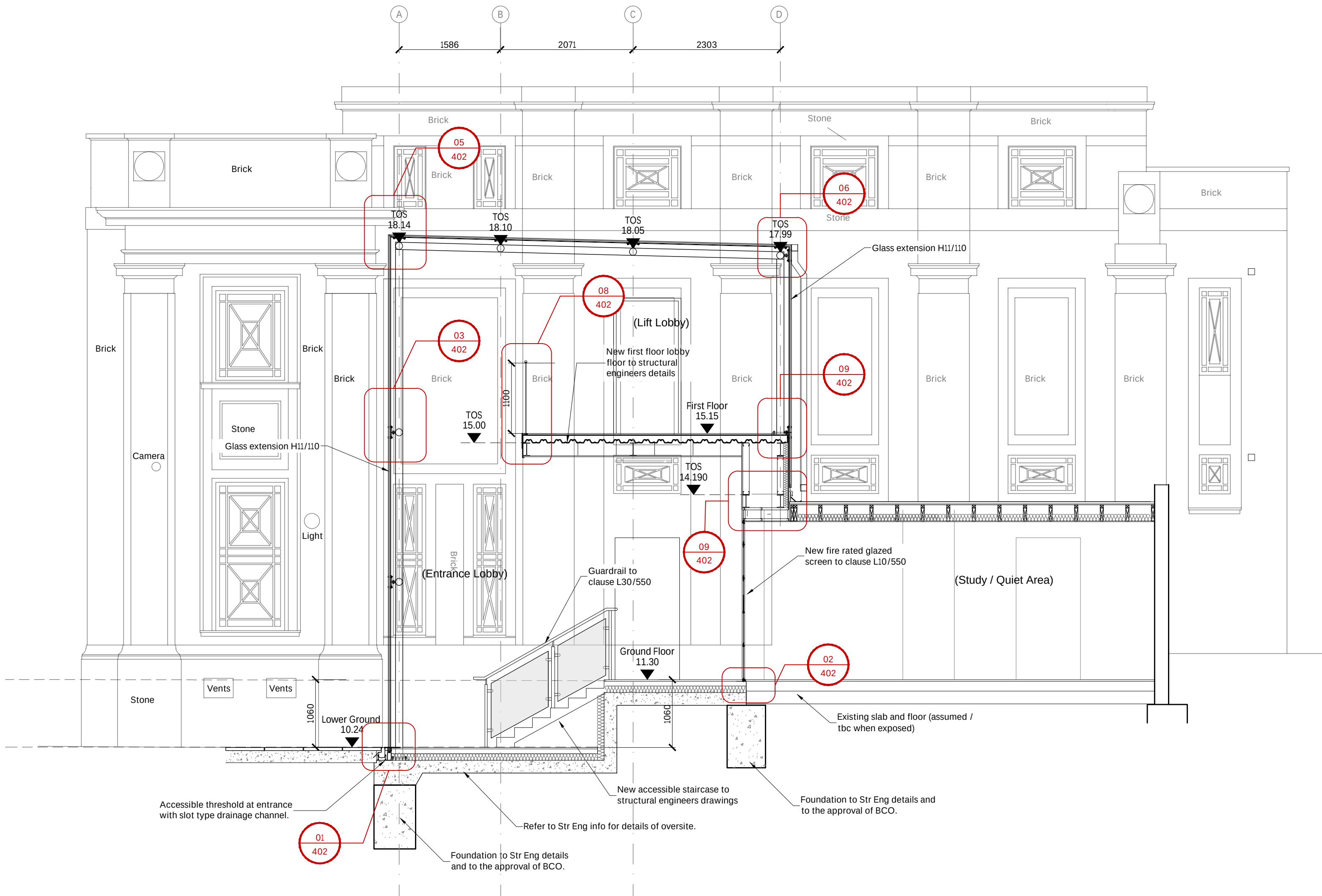
Section BB As Proposed
