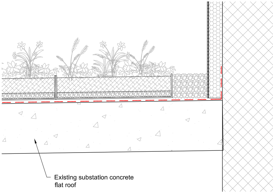
WALLBARN M-TRAY MODULE IMAGE SCALE N/A
