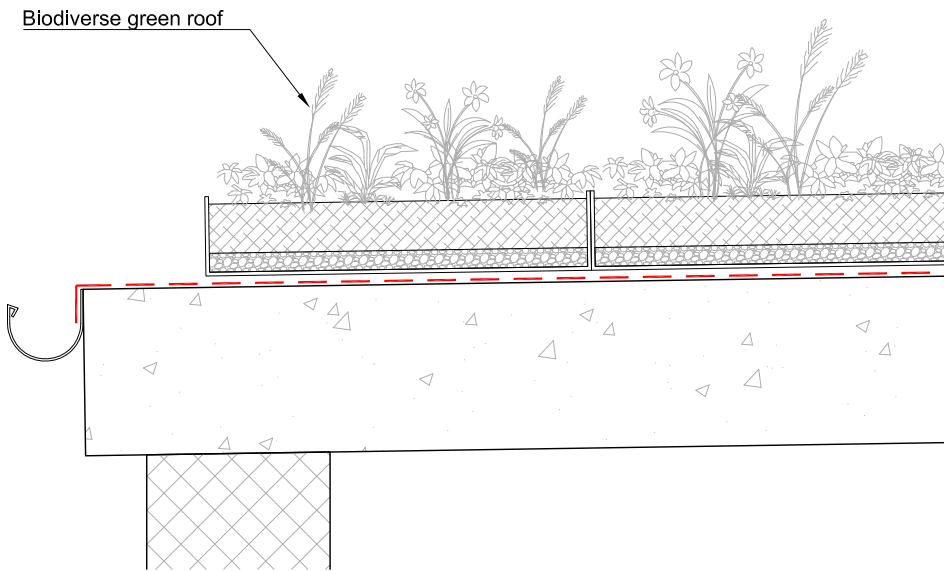
GREEN ROOF SECTION DETAIL SCALE 1:10 @ A3
