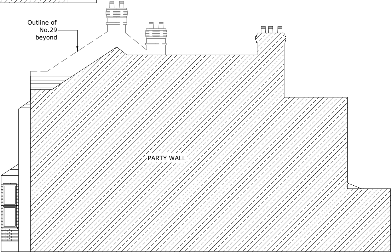
PROPOSED SIDE ELEVATION - B SCALE 1:100
