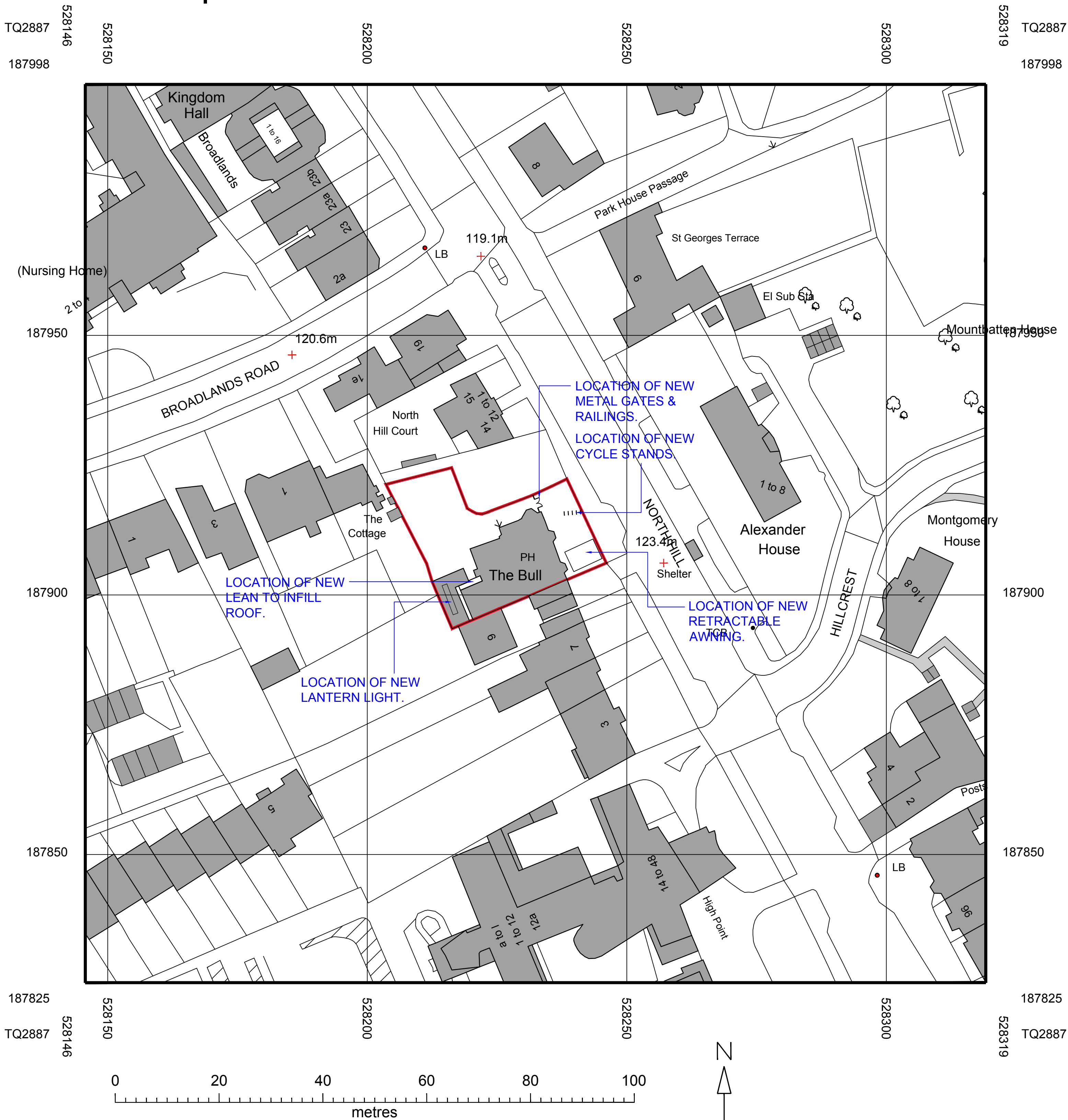
BLOCK PLAN. scale 1:500.
