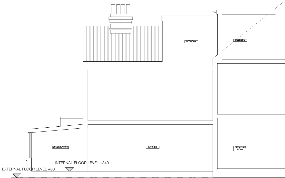
Section AA 1:100
