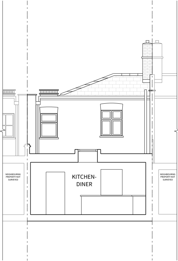
EXISTING SHORT SECTION A
