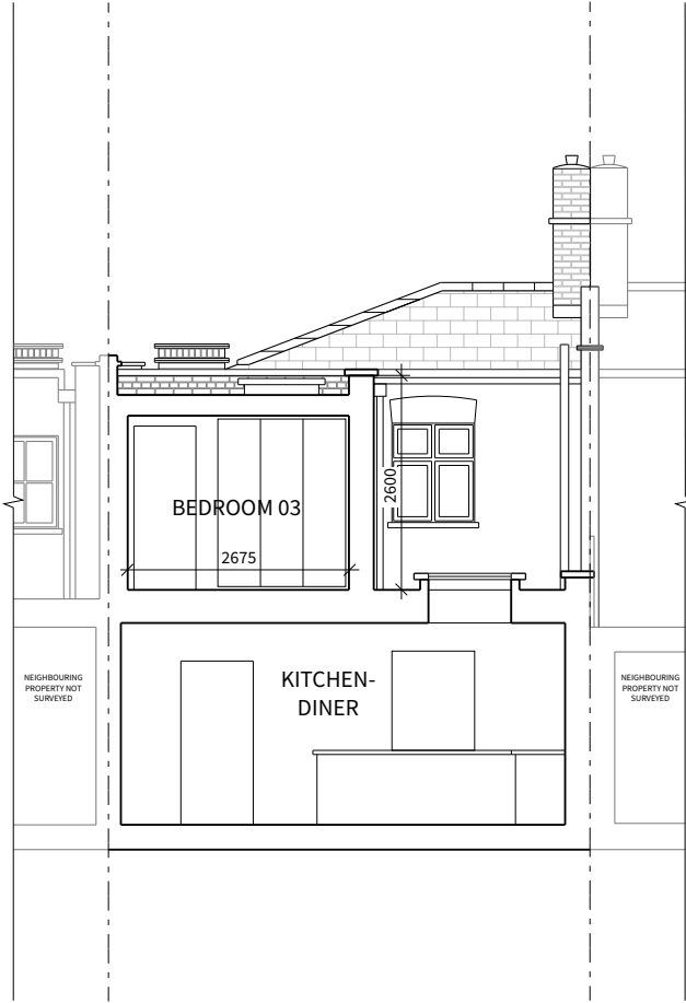
PROPOSED SHORT SECTION A
