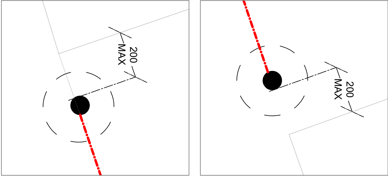
SP 11A Detail Scale 1:10
