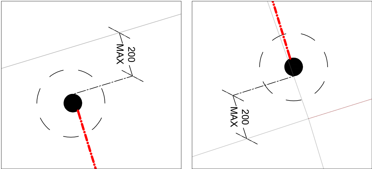
SP 2A Detail Scale 1:10
