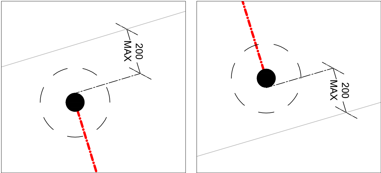
SP 4A Detail Scale 1:10
