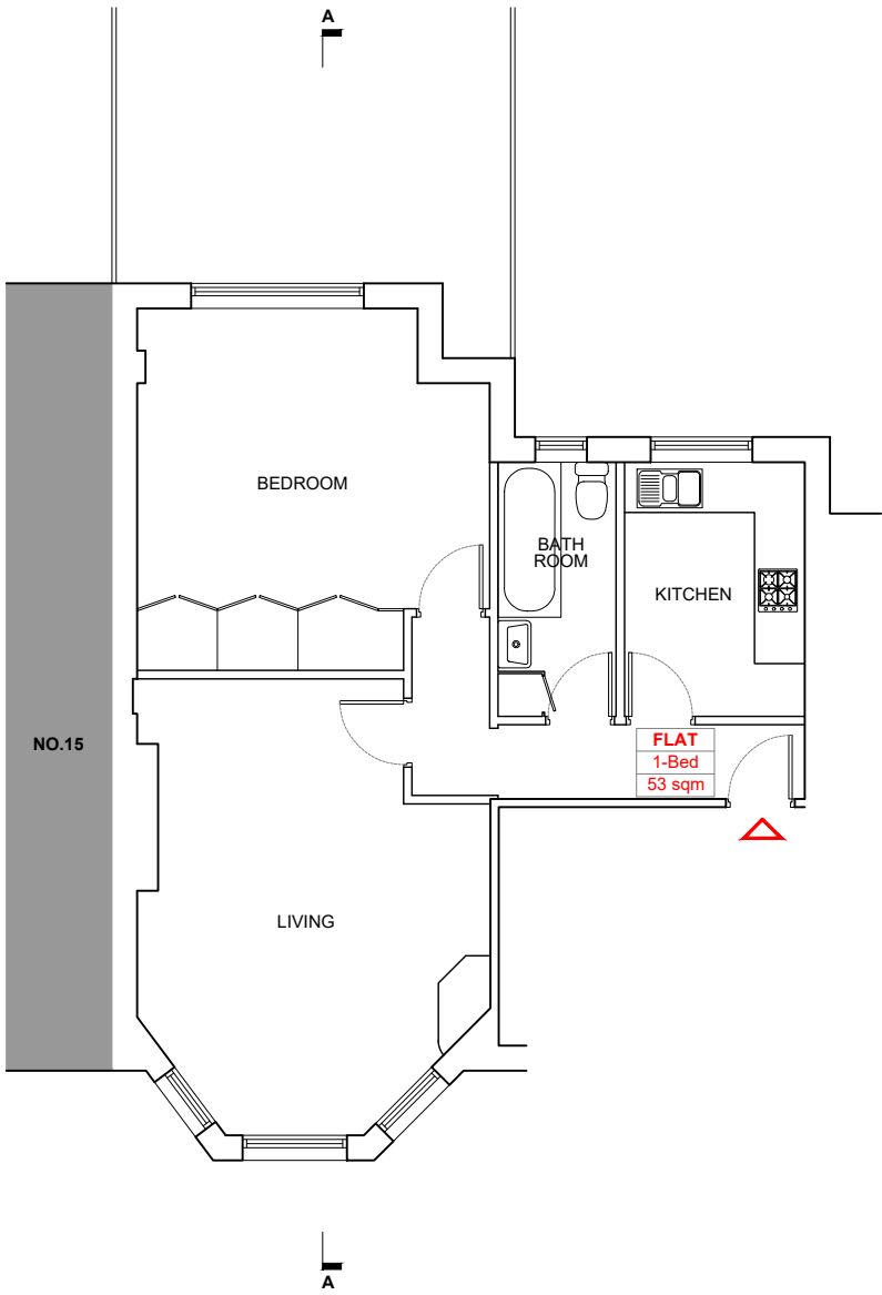
Existing Upper Ground Floor Plan
