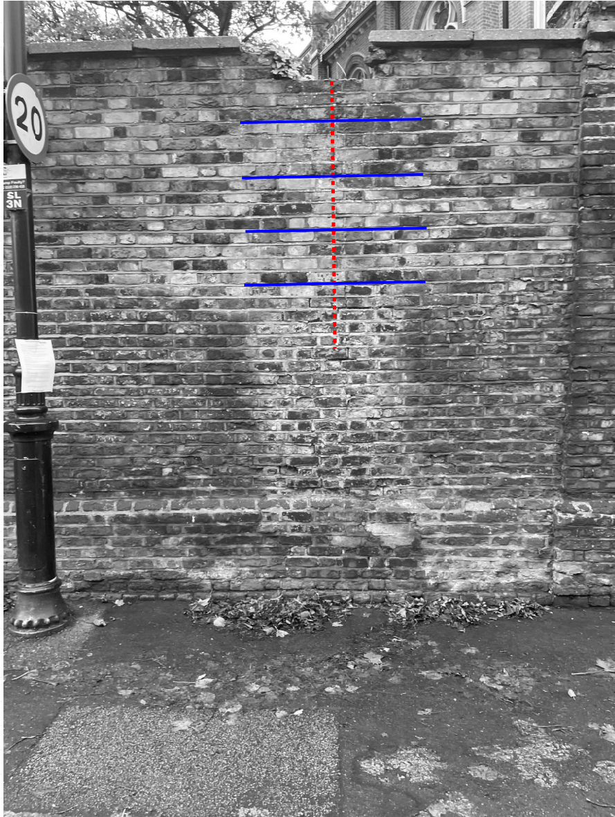
Helibar repair location on panel and detail as SK20
