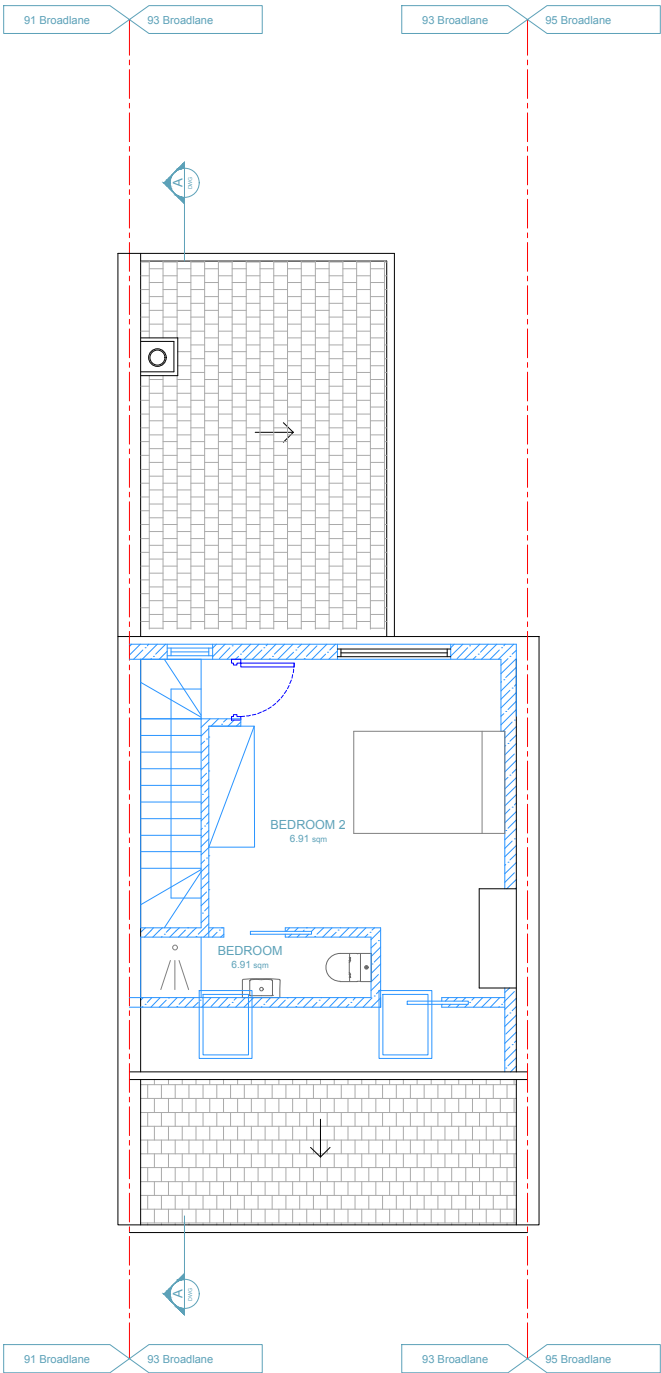
PROPOSED LOFT FLOOR PLAN
