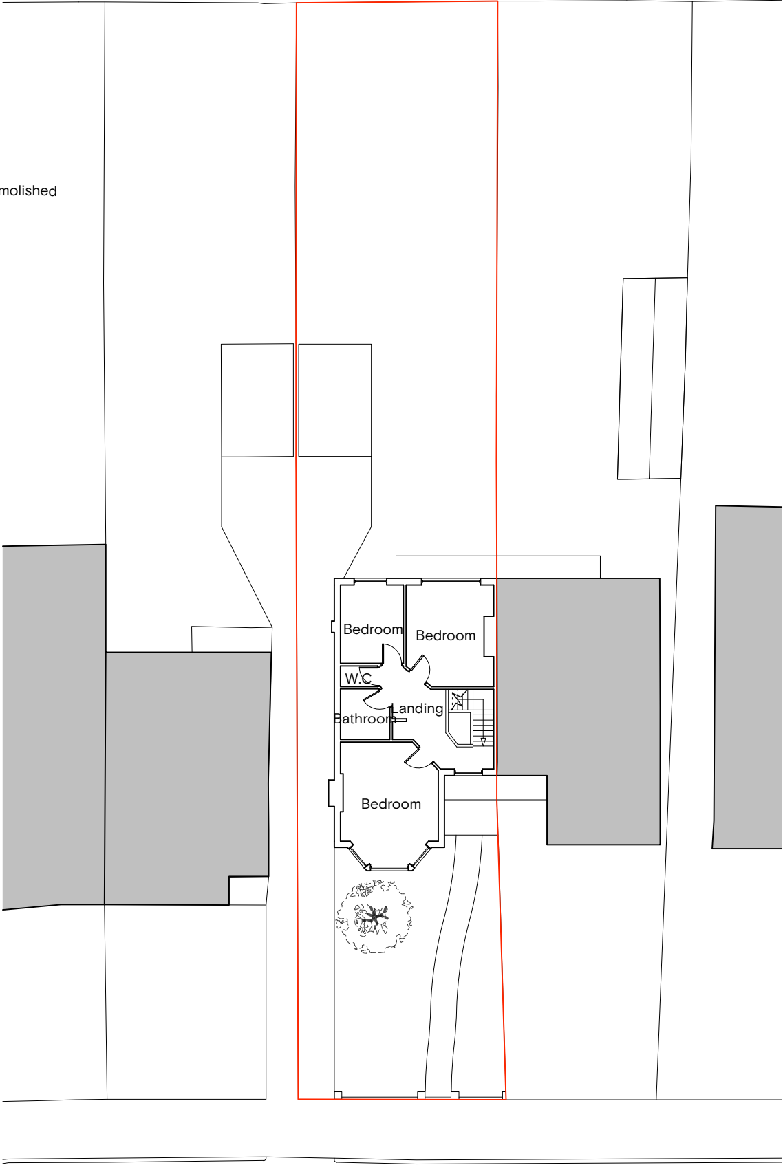
Existing First Floor Woodfield Way
