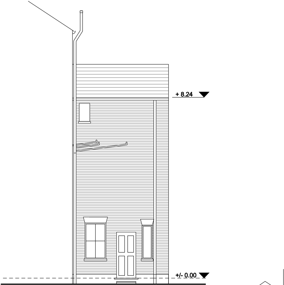
SOUTH ELEVATION
