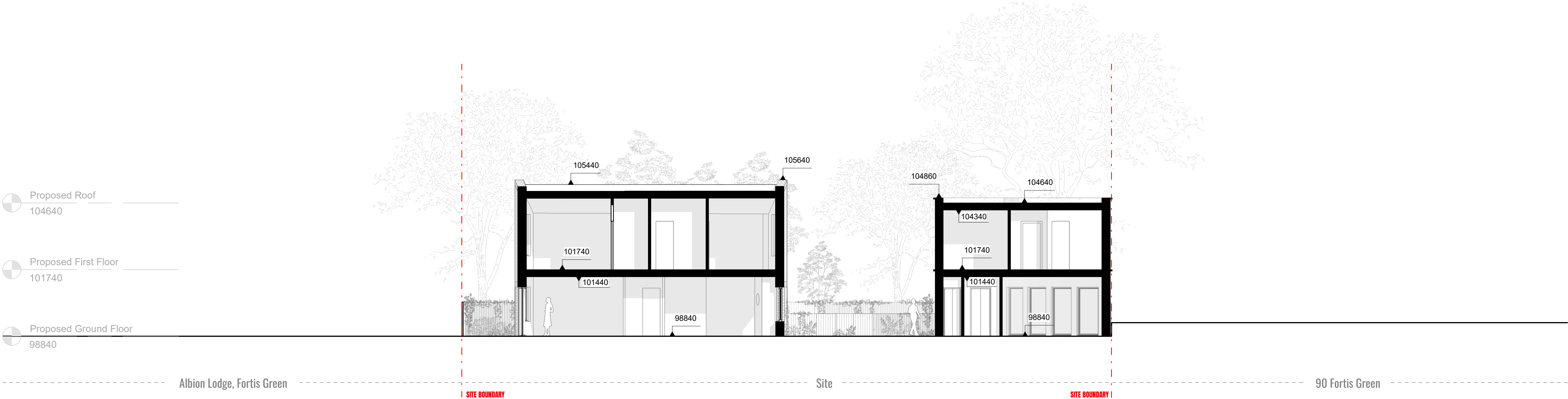
1 Section B-B 1:100
