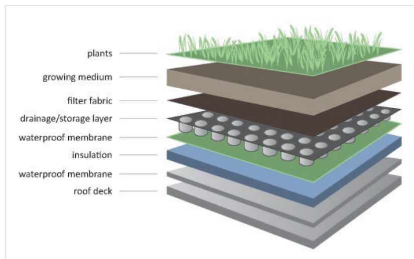
Figure 9: Indicative Build-up of Brown Roof
