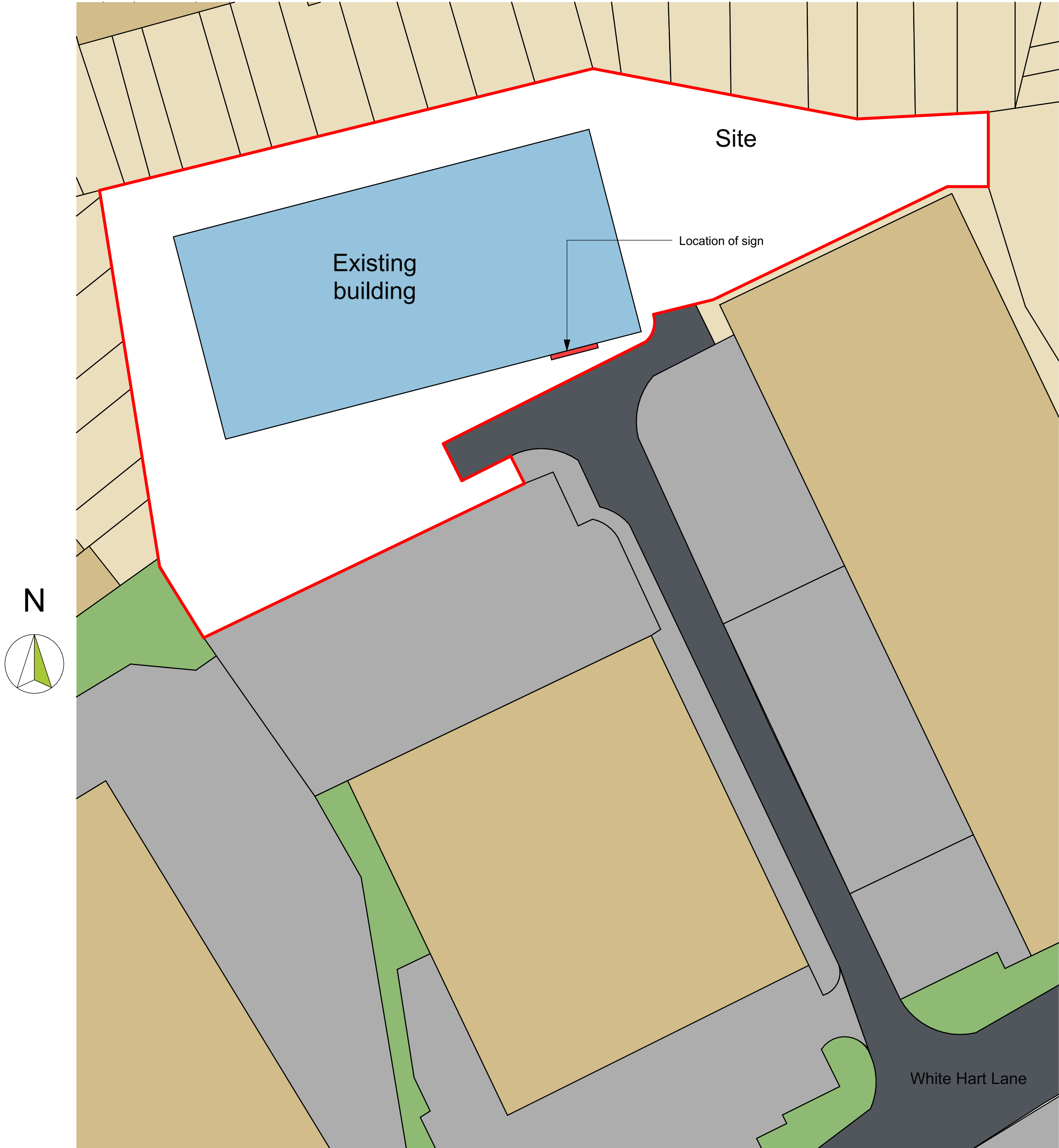
Block Plan 1:500
