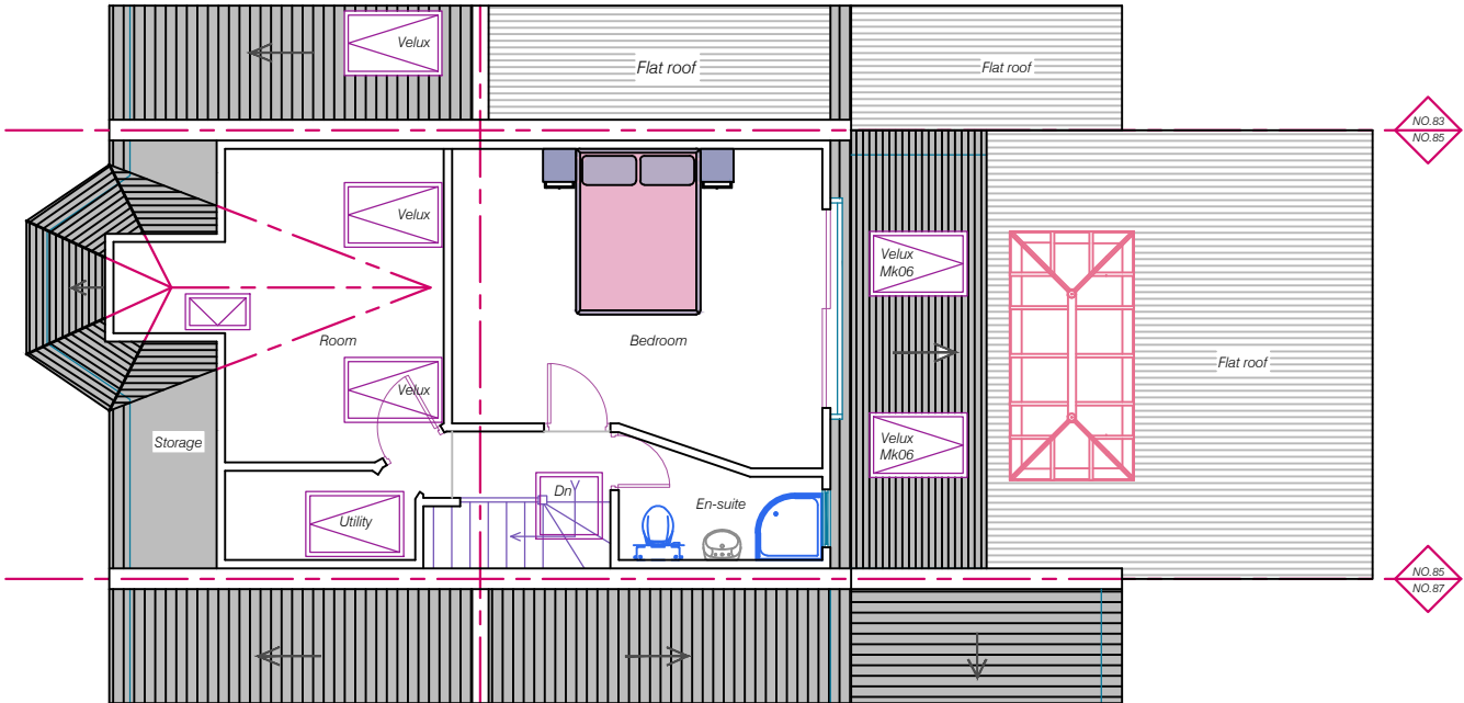
EXISTING LOFT PLAN
