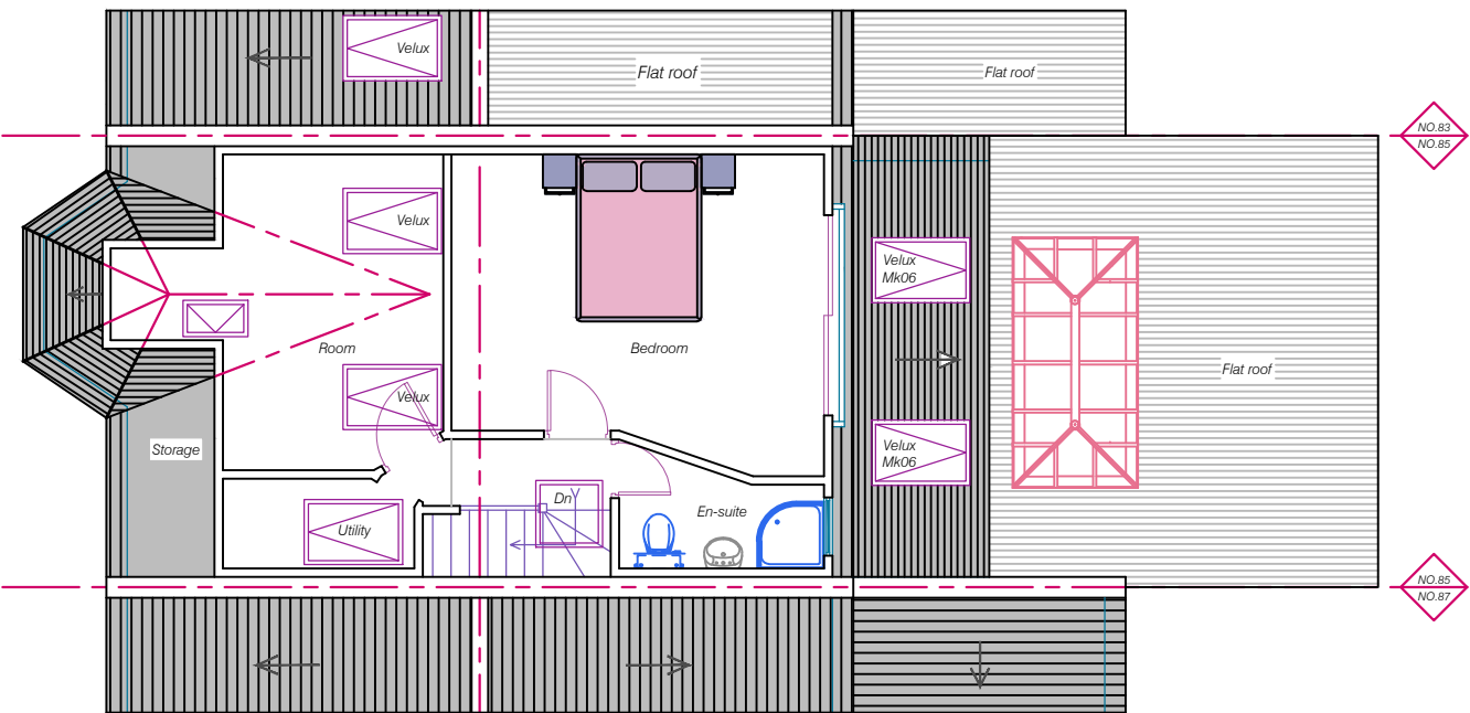
PROPOSED LOFT PLAN
