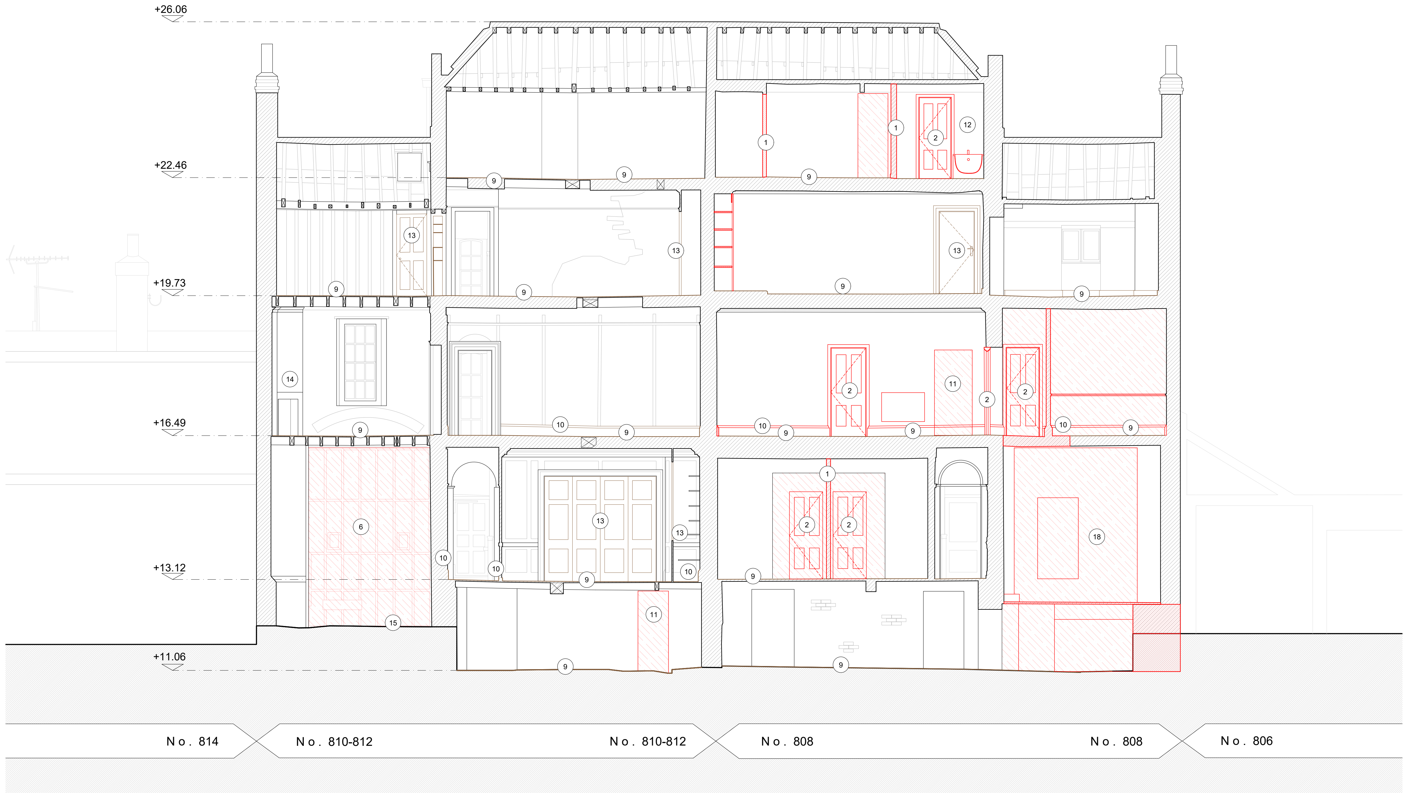
01 SECTION AA - EXISTING + STRIP OUT 92200 Scale 1:50
