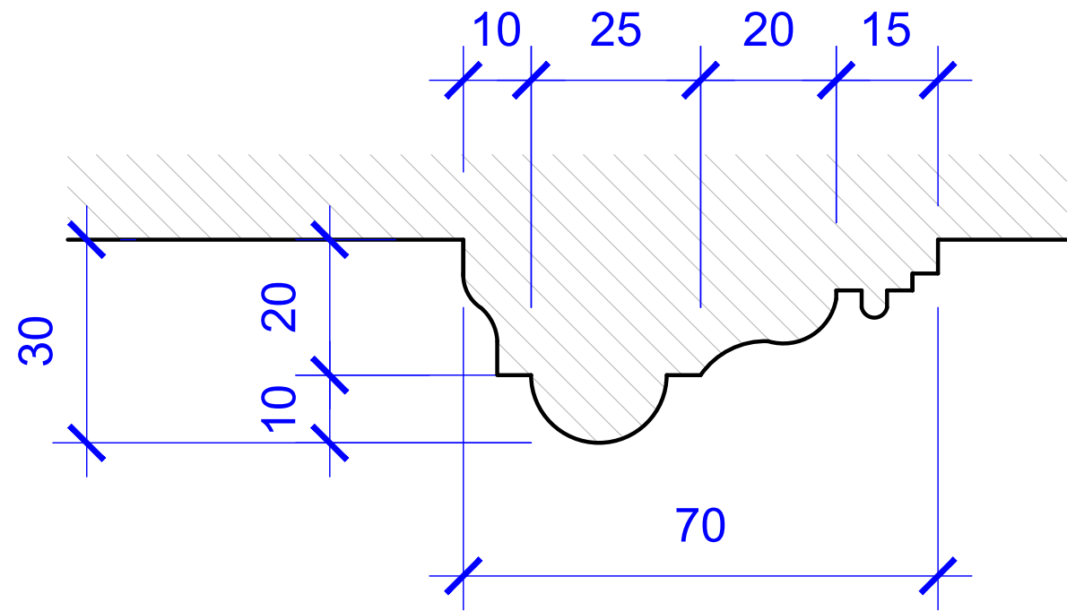
02 FIREPLACE TYPE 01 - MOULDING Scale 1:1
