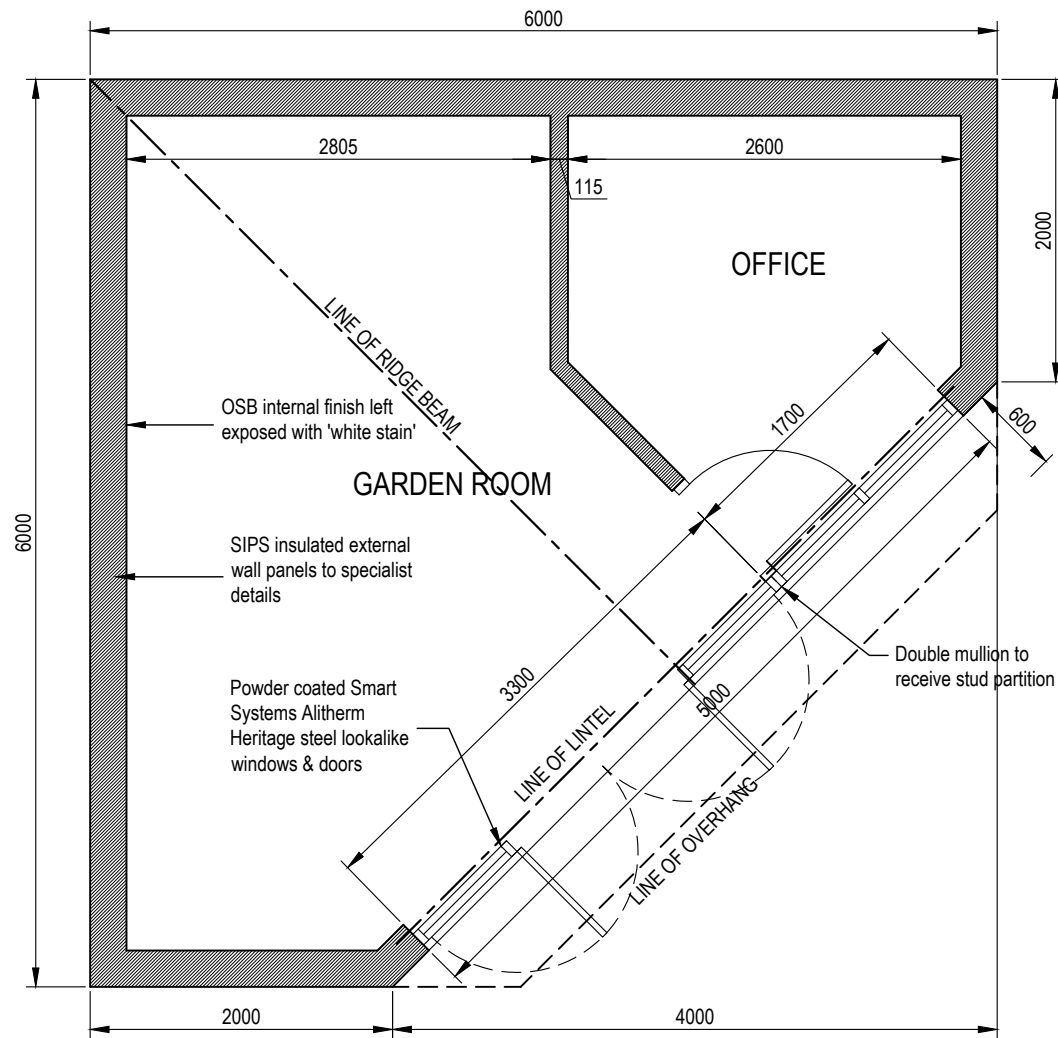
FLOOR PLAN
