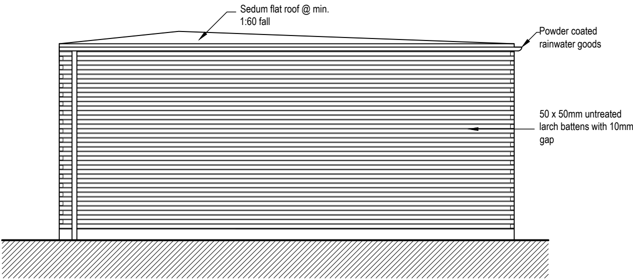
REAR ELEVATION 1
