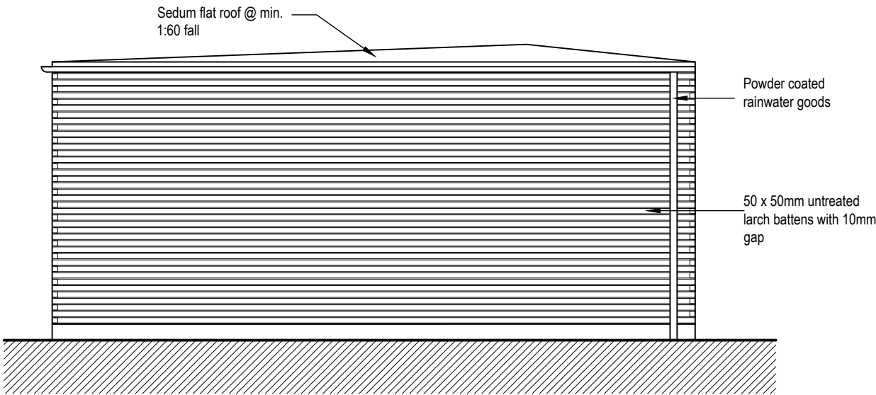
REAR ELEVATION 2
