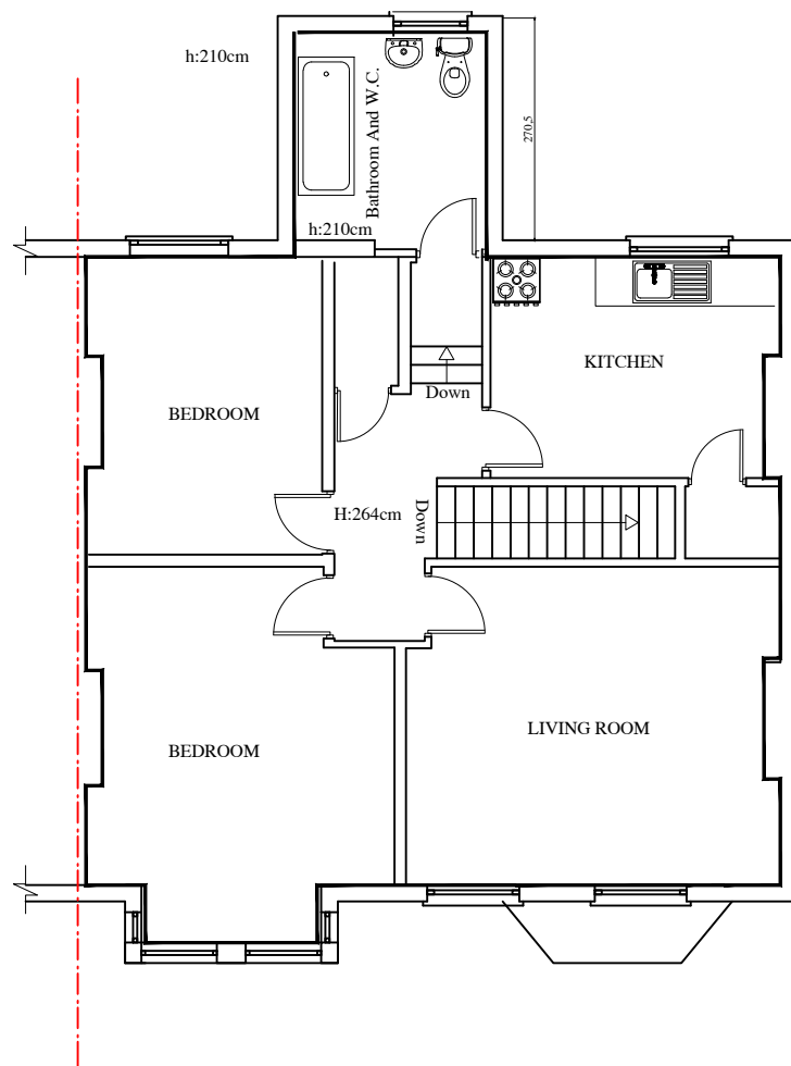
EXISTING FIRST FLOOR PLAN FLOOR AREA:71m²
