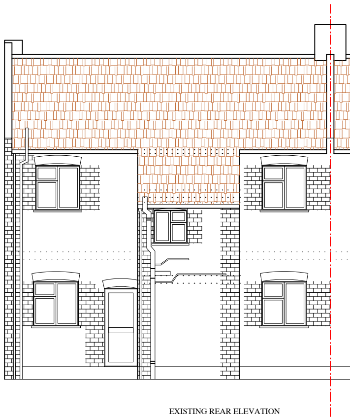
EXISTING REAR ELEVATION NO ALTERATION
