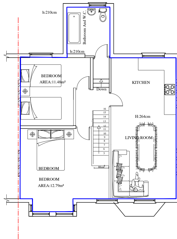
PROPOSED FIRST FLOOR PLAN FLOOR AREA:72m²
