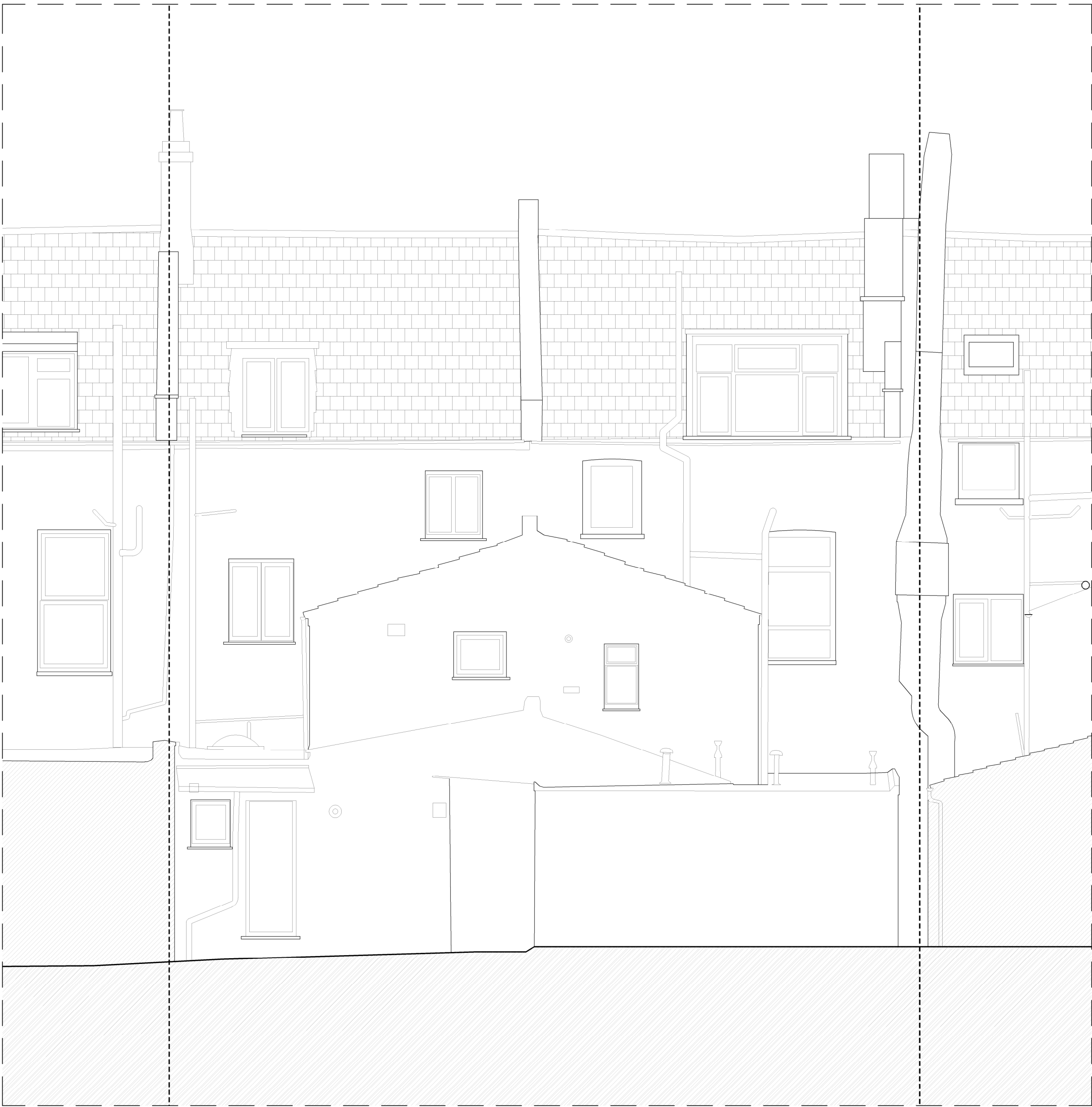
Rear Elevation
