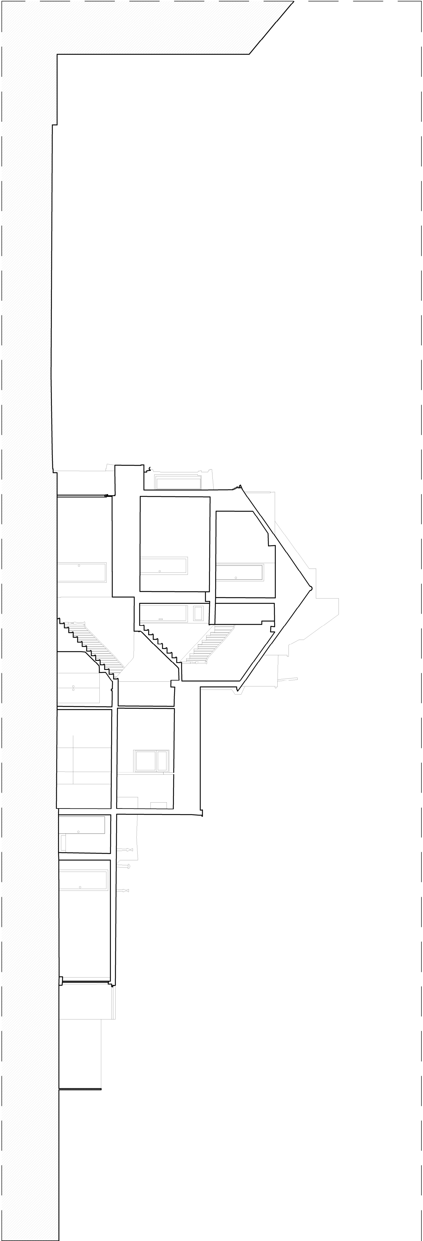
Section AA
