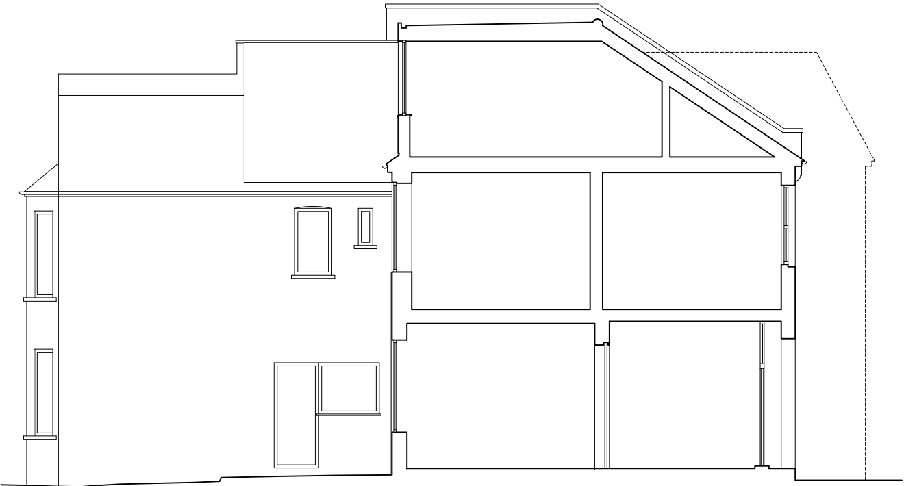
SECTION AS EXISTING
