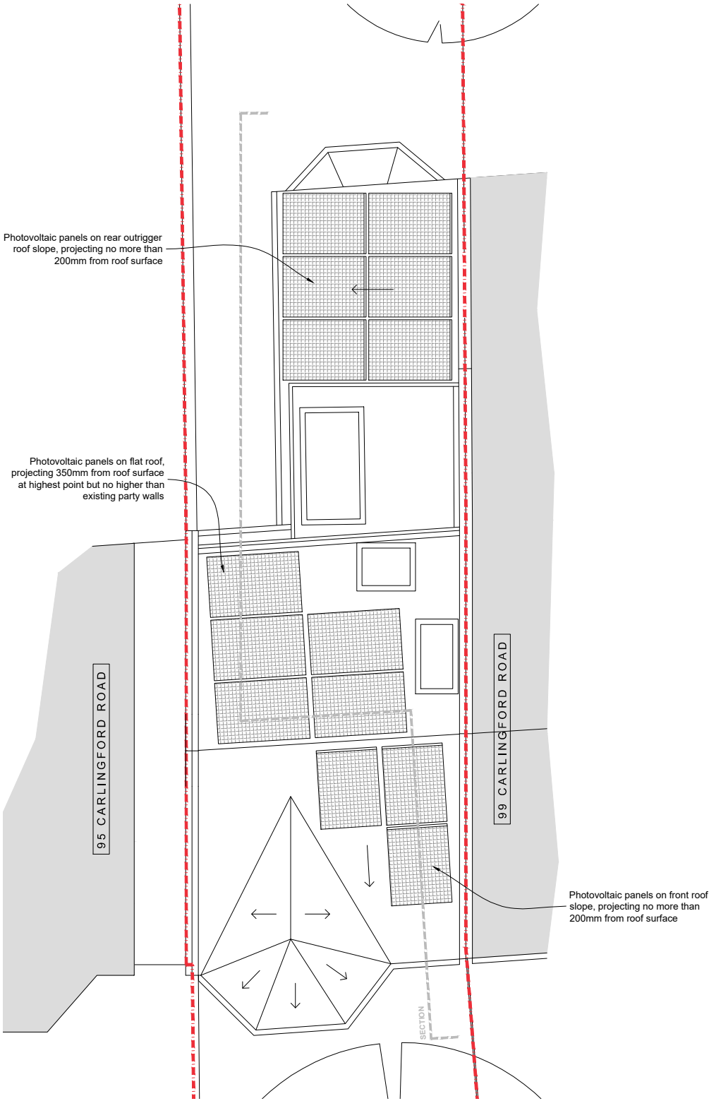
ROOF PLAN AS PROPOSED
