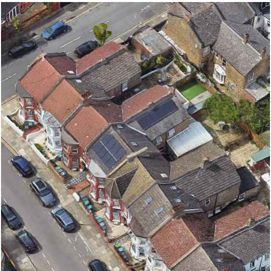
35 CARLINGFORD ROAD PV panels on front and rear outrigger roof slopes
