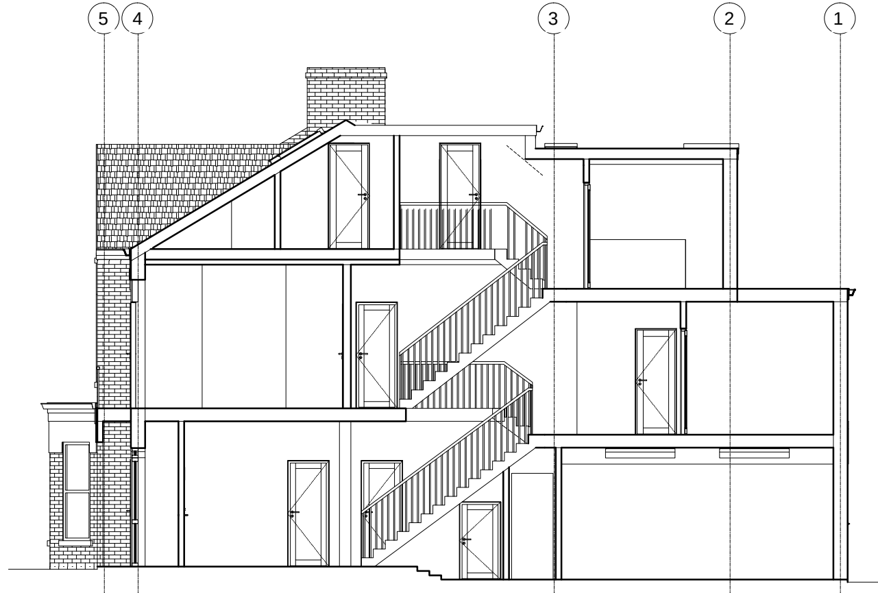
PROPOSED SECTION
