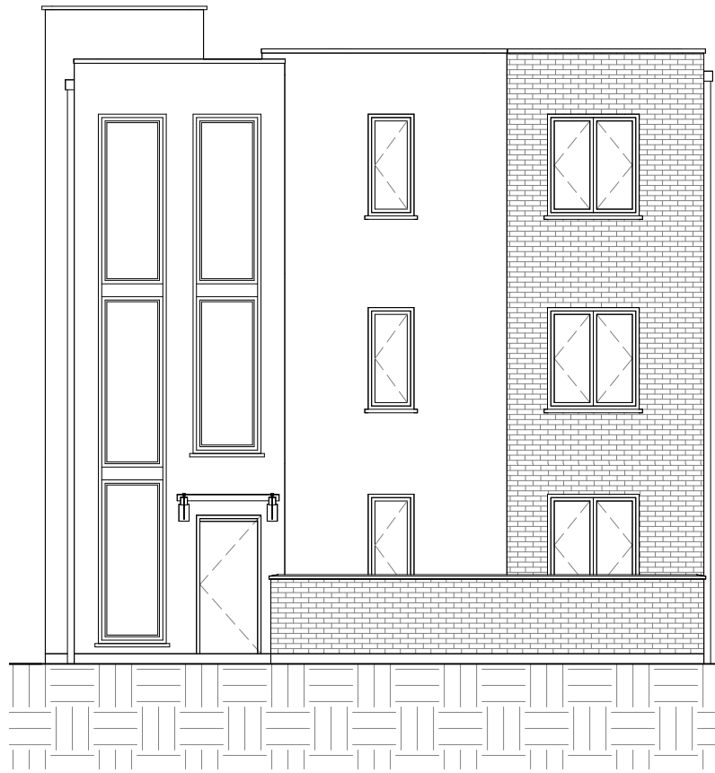
South Elevation as Existing 1 : 100
