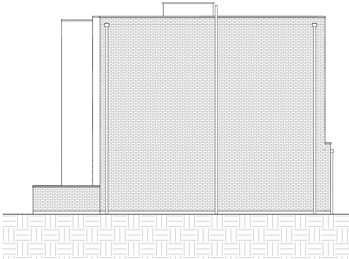
East Elevation as Existing 1 : 100
