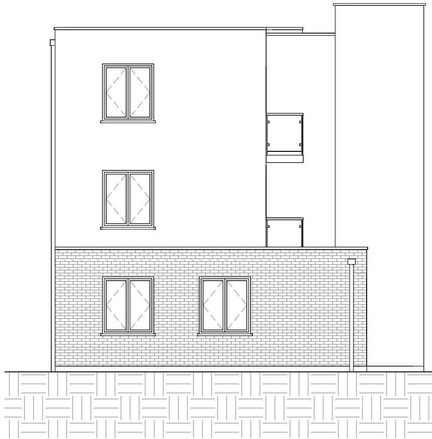
North Elevation as Existing 1 : 100
