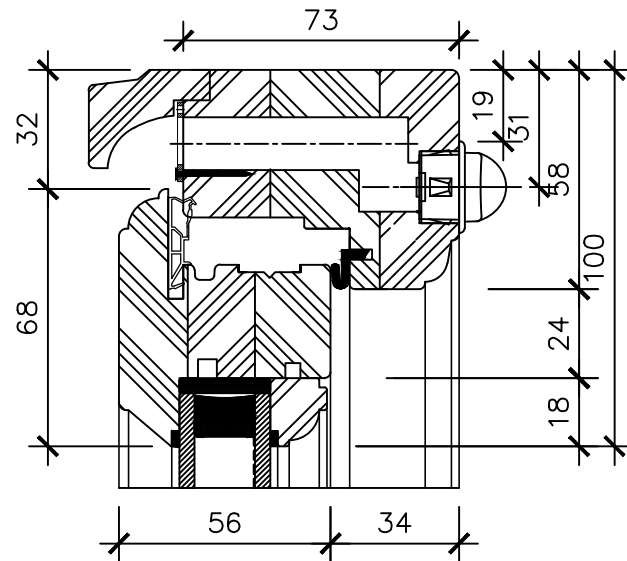
Traditional Lipped Casement Window Frame & Sash Head (Standard 58mm Head With Vent)
