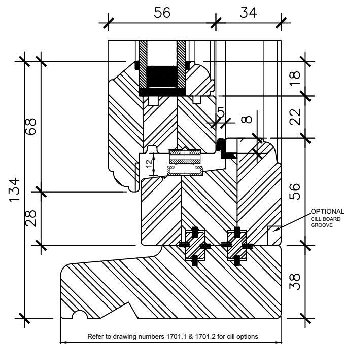
Traditional Lipped Casement Window Frame & Sash Cill (With Subcill)
