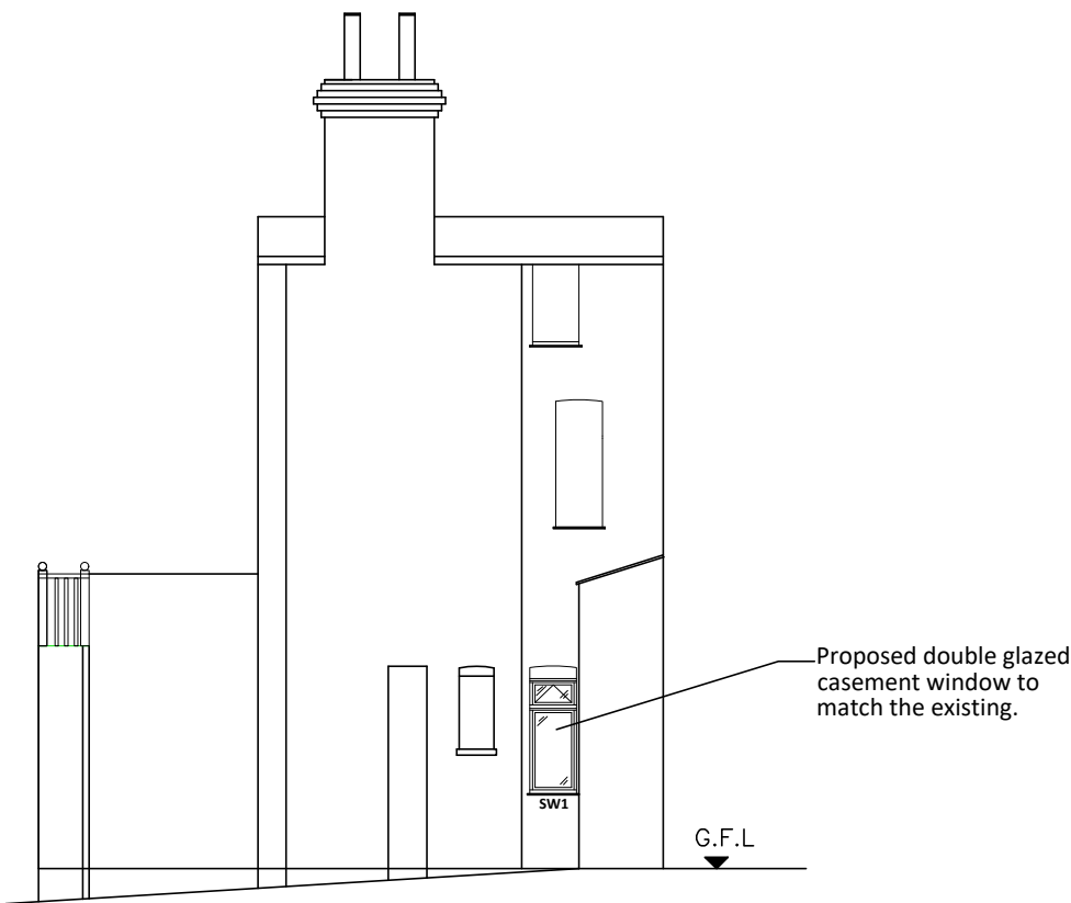
PROPOSED SIDE ELEVATION No. 71 HILLFIELD PARK
