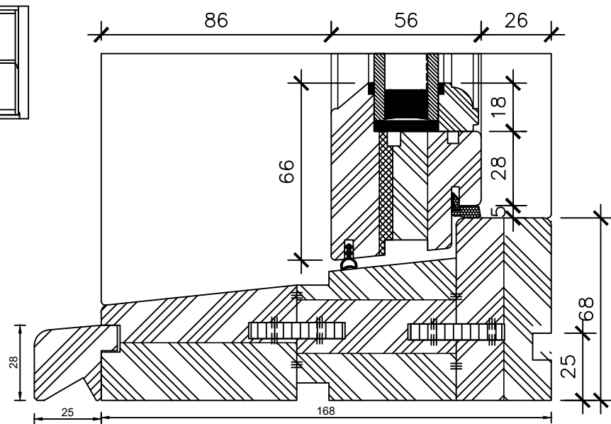
Traditional Sliding Sash Cords & Weights Frame & Sash Cill
