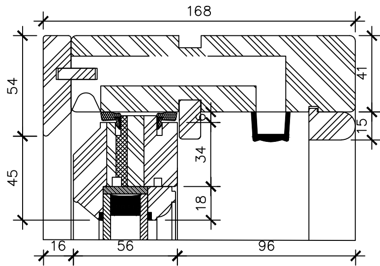
Traditional Sliding Sash Cords & Weights Frame & Sash Head (With Vent)
