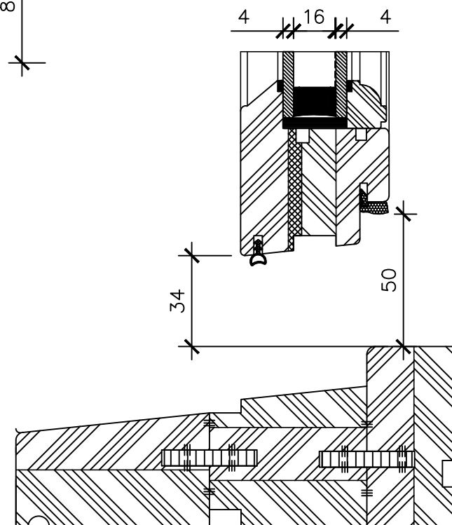
Traditional Sliding Sash Cords & Weights Standard Restrictor Position (50mm)
