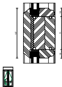
Traditional Open in Flush French Door Mid Rail
