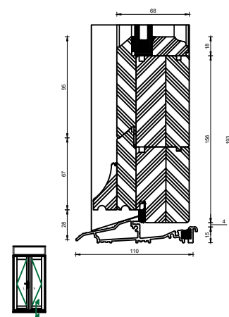
Traditional Open In Flush French Door Mobility Thresh
