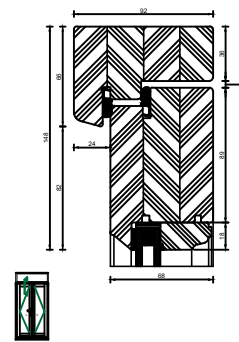
Traditional Open In Flush French Door Frame & Leaf Head
