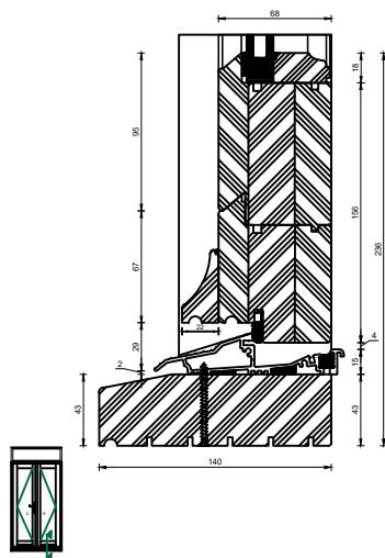
Traditional Open In Flush French Door Standard Thresh (140x43mm)
