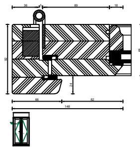
Traditional Open In Flush French Door Frame & Leaf Jamb
