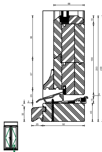
Traditional Open In Flush French Door Coupling Thresh
