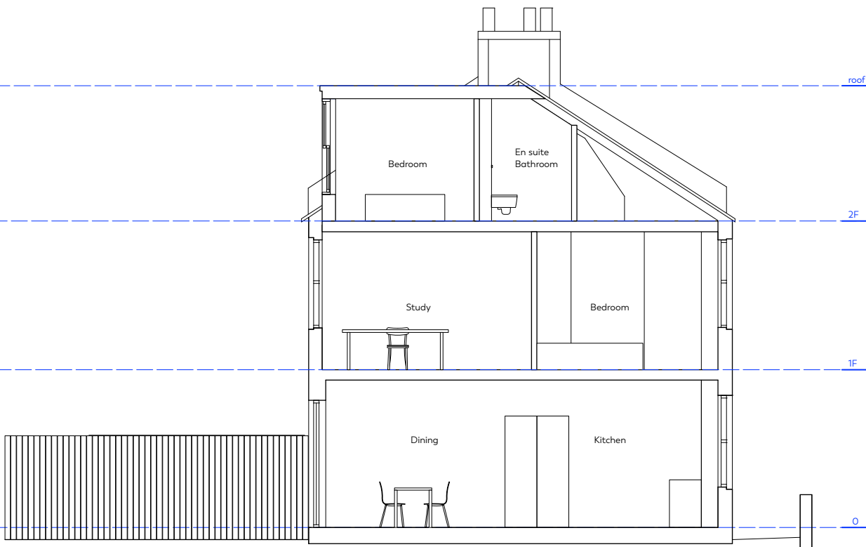
Proposed Section 1
