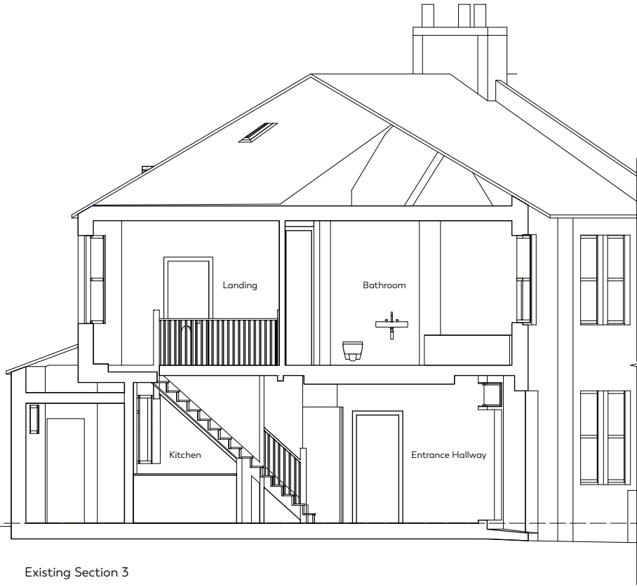
Existing Section 3
