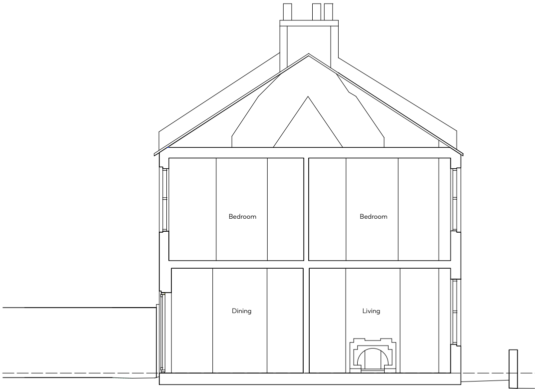
Existing Section 1
