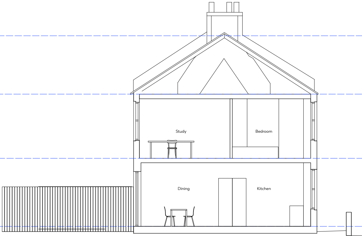
Proposed Section 1
