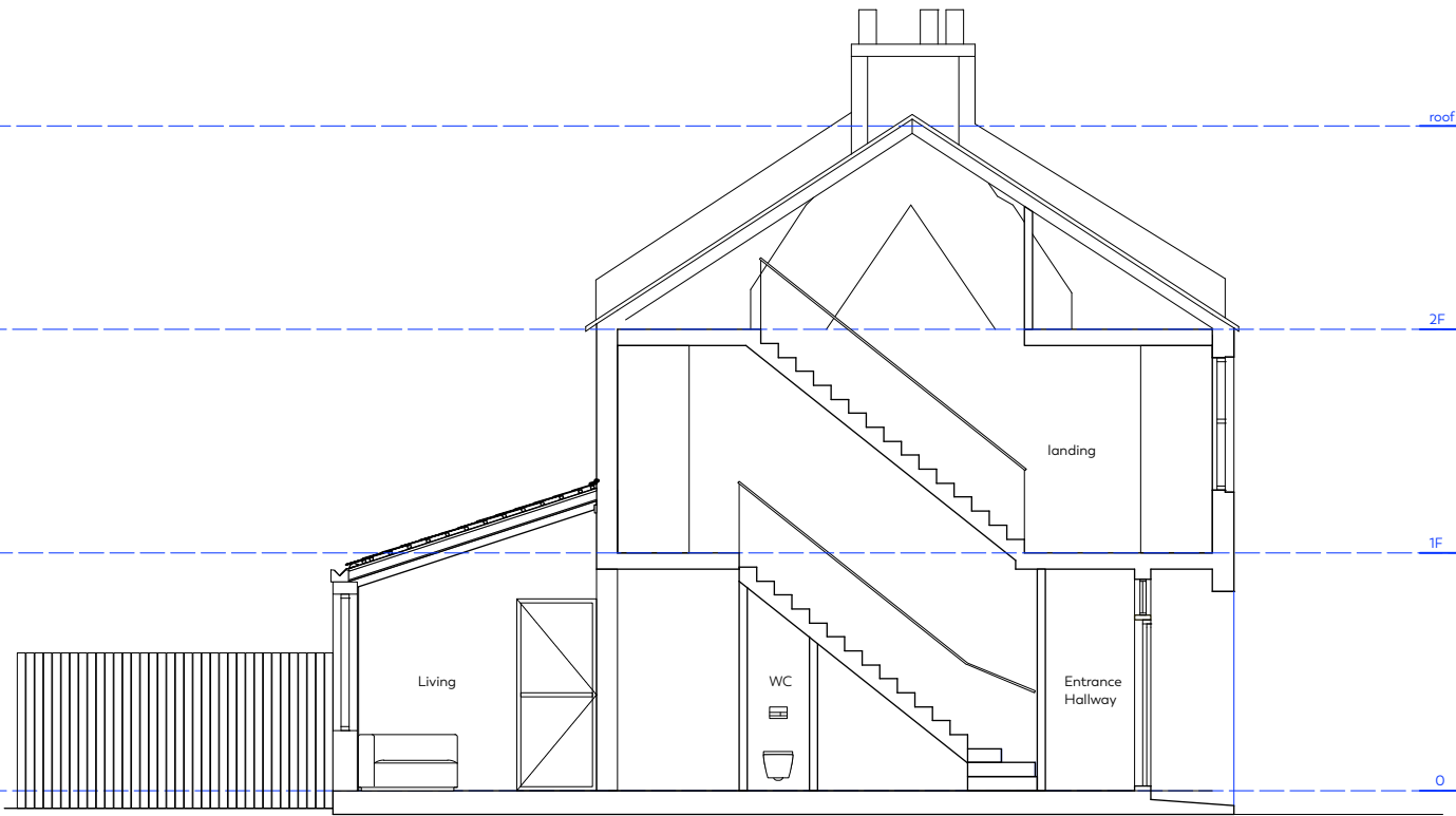
Proposed Section 3
