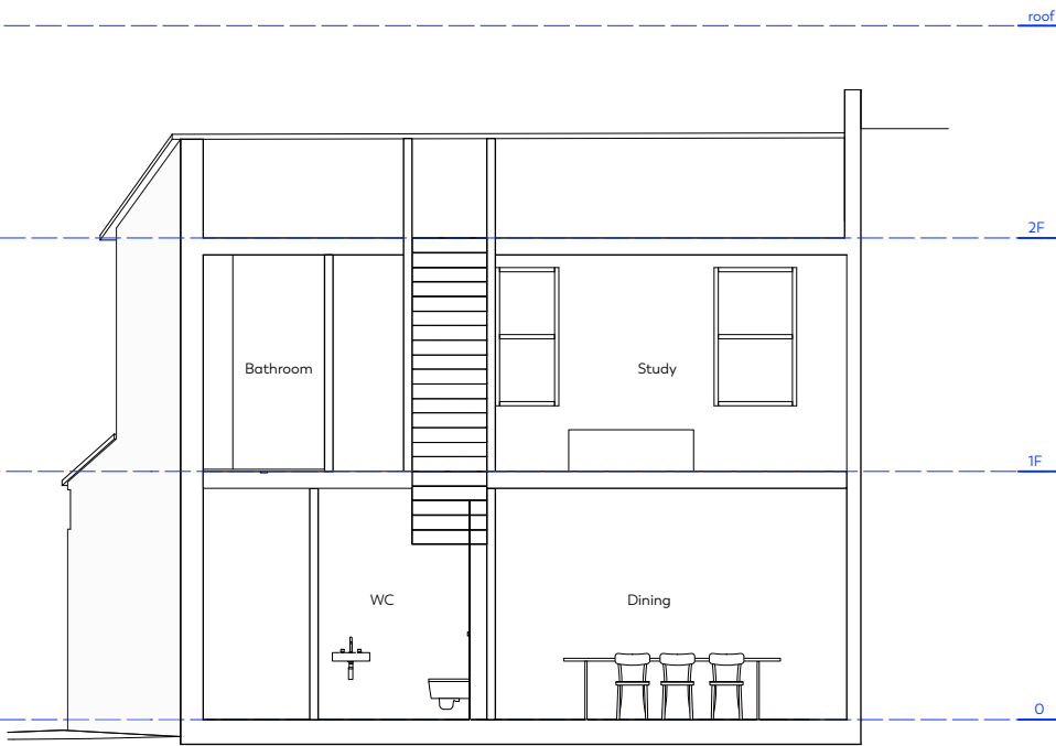
Proposed Section 2
