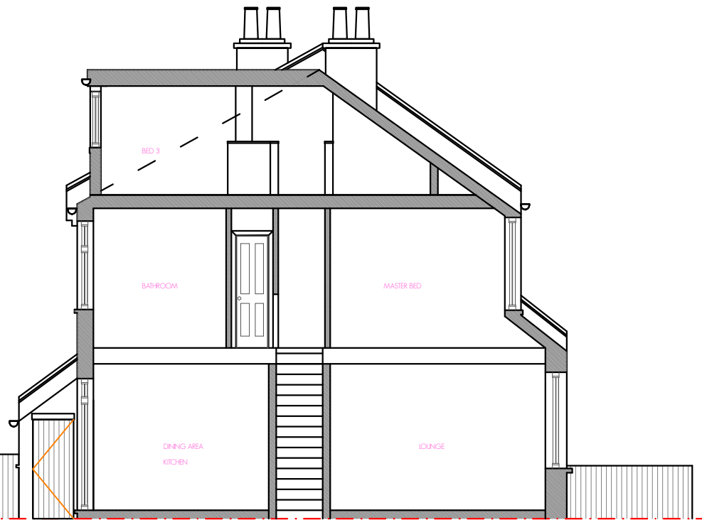
SECTION Existing
