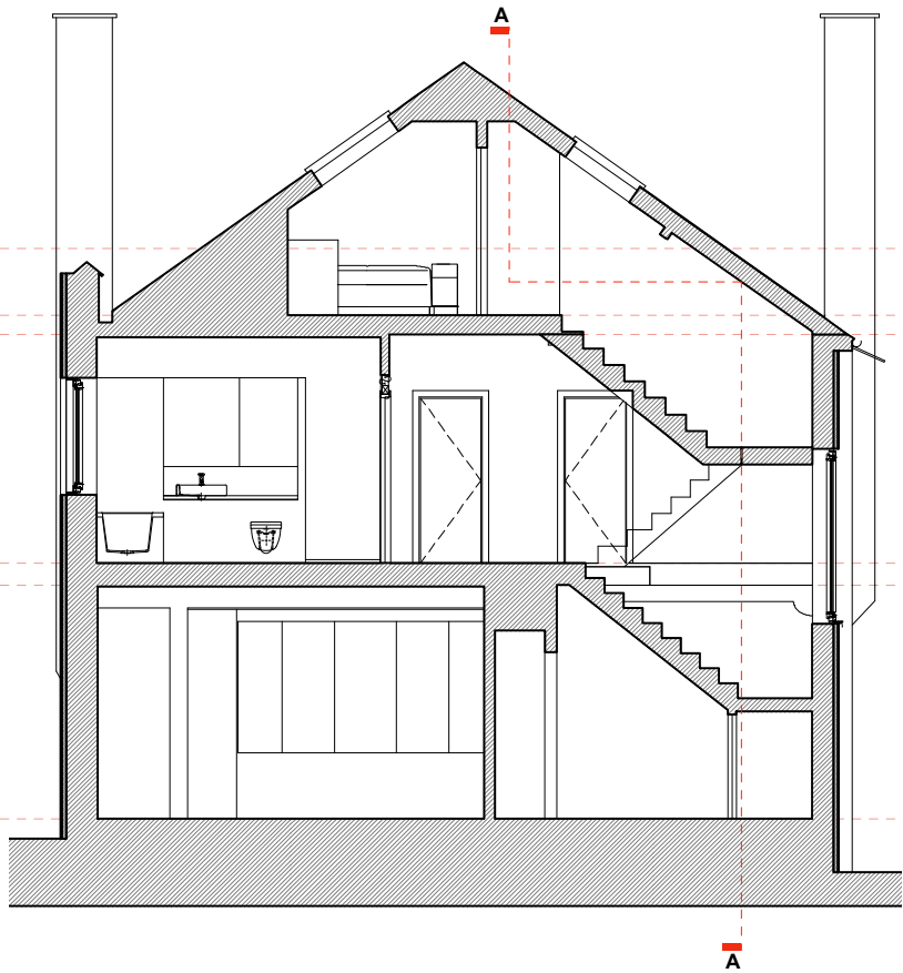
PROPOSED SECTION BB
