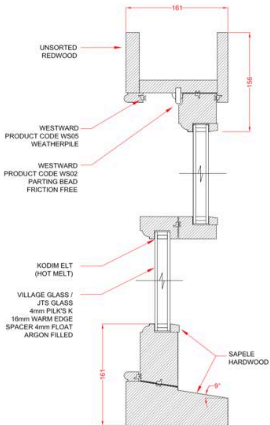
HEAD AND STILE ELEVATION NTS
