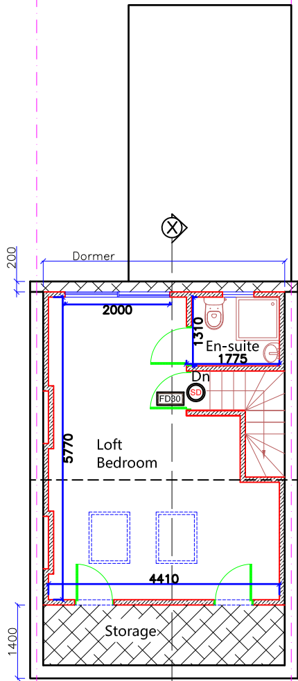
Proposed Loft Floor Plan
