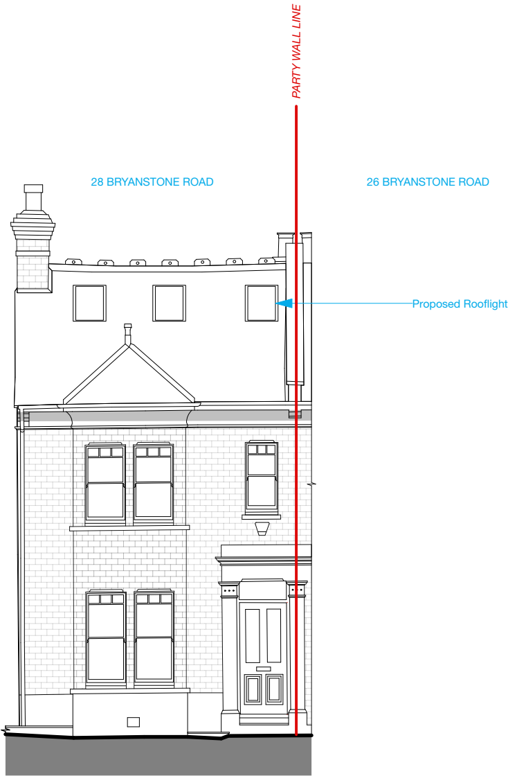
2 Proposed Front Elevation 1:100
