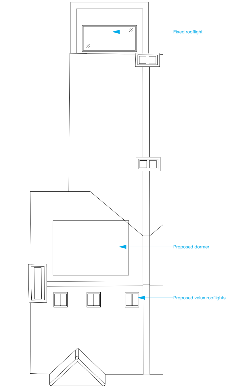
1 Proposed Roof Plan 1:100
