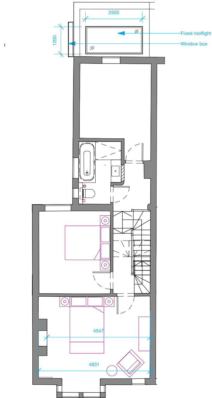
1 Proposed First Floor Plan 1:100
