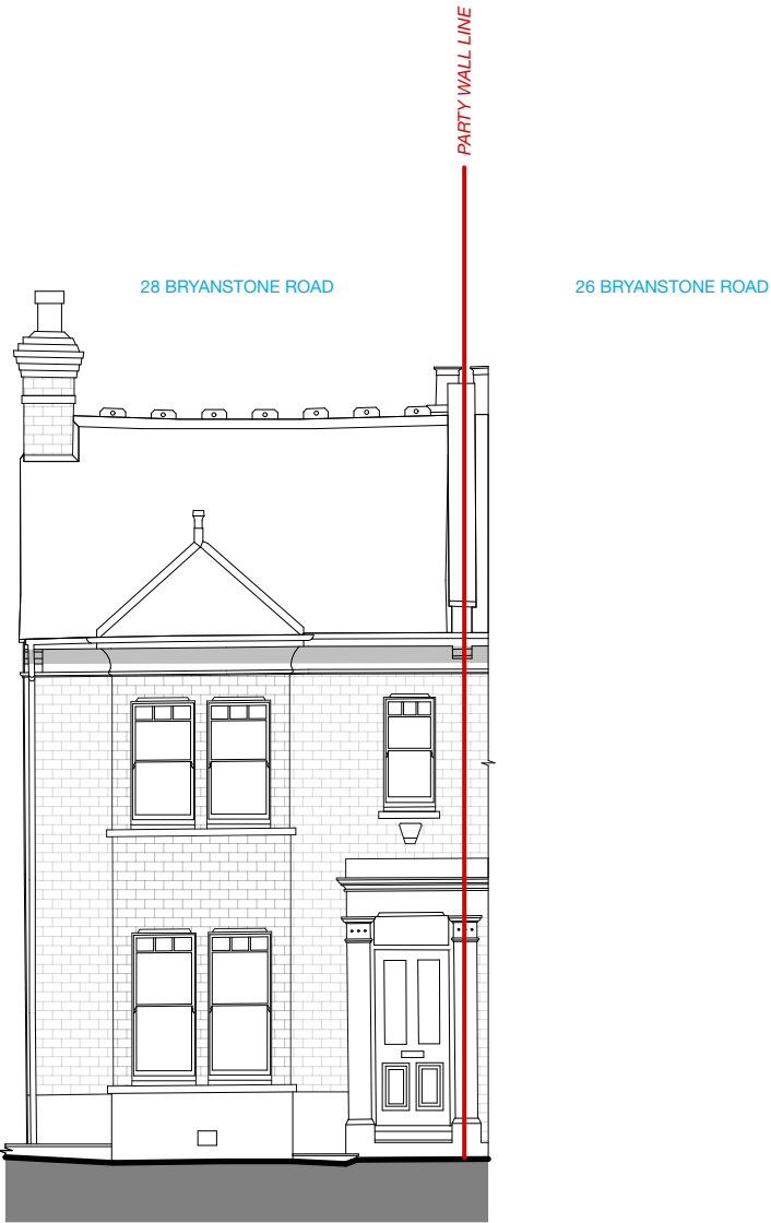
2 Existing Front Elevation 1:100
