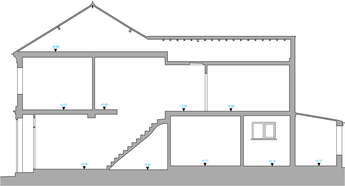
2 Existing Section AA 1:100
